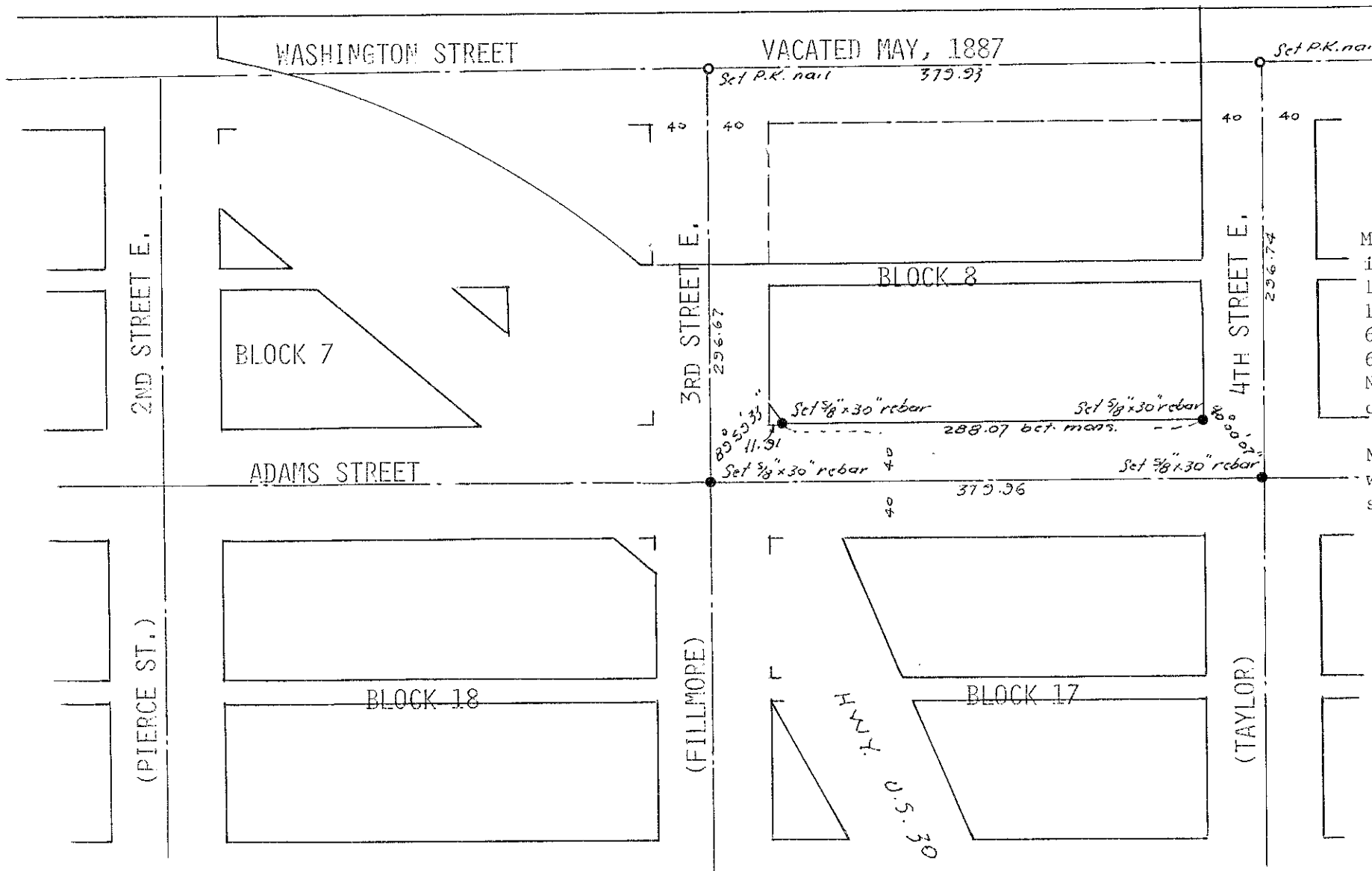
MAP OF SURVEY THE SOUTH LINE OF BLOCK 8, HUNTINGTON TOWNSITE For the City of Huntington, Oregon Surveyed June 4, 1981 Scale: 1" = 100'
