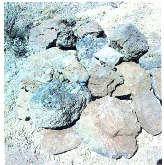
Set brass cap monument to within 8" of the surface in a mound of stone 3 feet at base around monument. Original stone is buried on the West side of monument.
