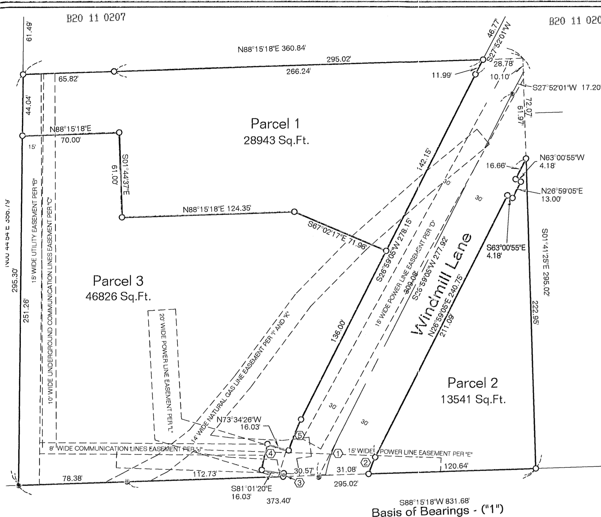
VARIOUS EXISTING UTILITY EASEMENTS SCALE: 1" = 40'
