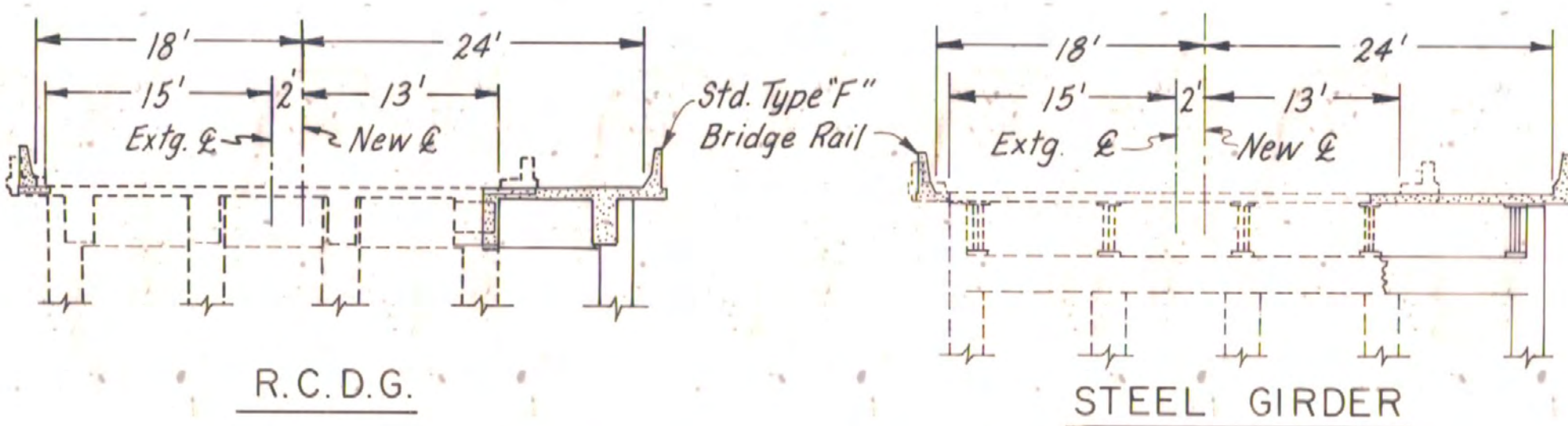
TYPICAL SECTIONS
